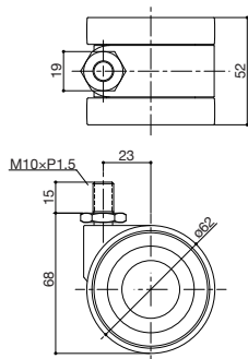
DF1-0MA-ZN2-062 ねじ込みタイプ Threaded stem type
