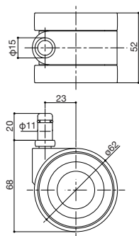
DF1-0MK-ZN2-062 差し込みタイプ Threaded stem type
